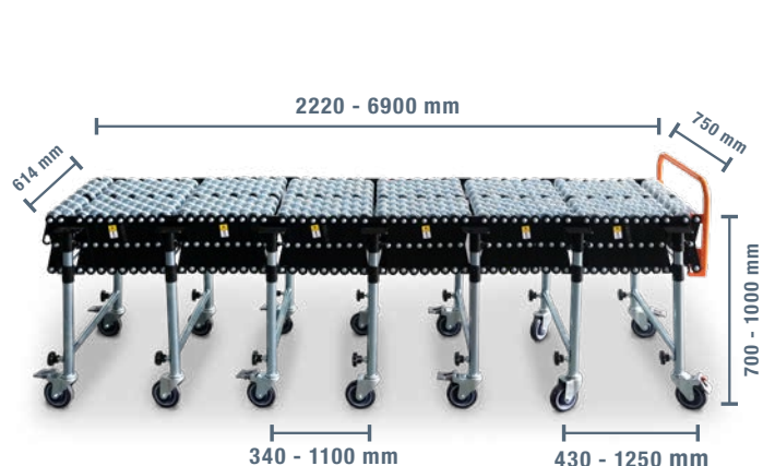
Measurements skatewheel conveyor
