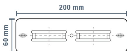
Support mural
